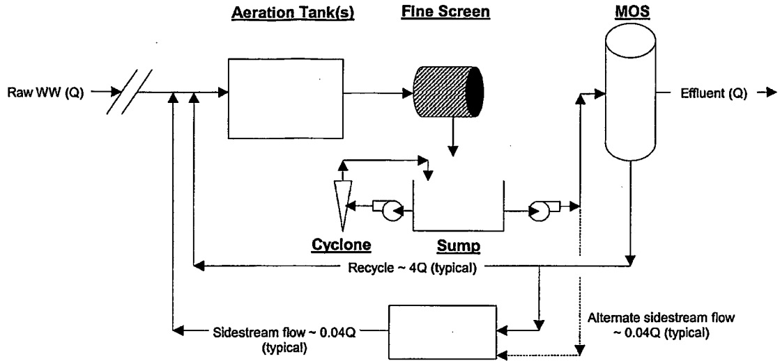
Figure 26 - Sidestream Anoxic Reactor
